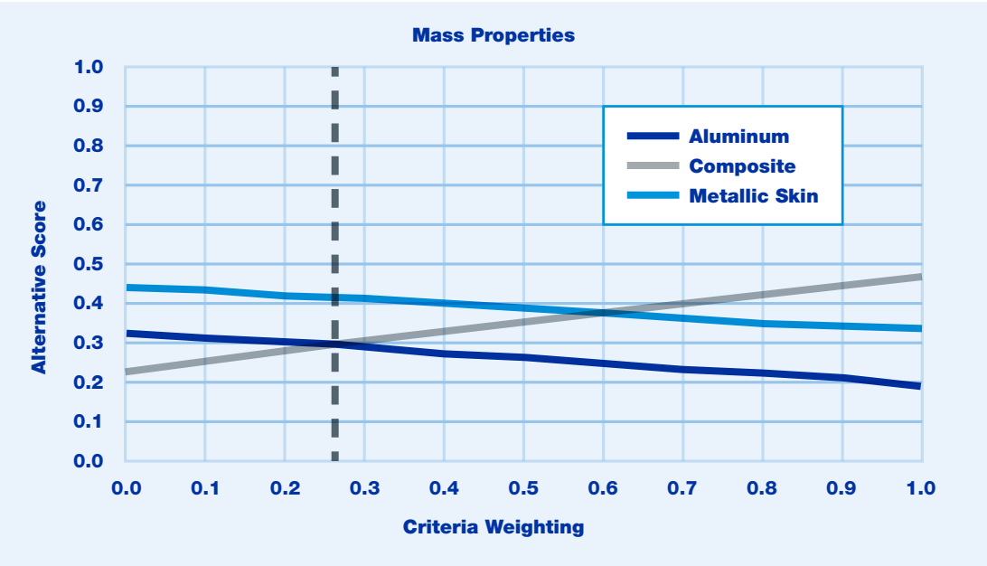
FIGURE 4. Criteria-weighting sensitivity analysis curve example
