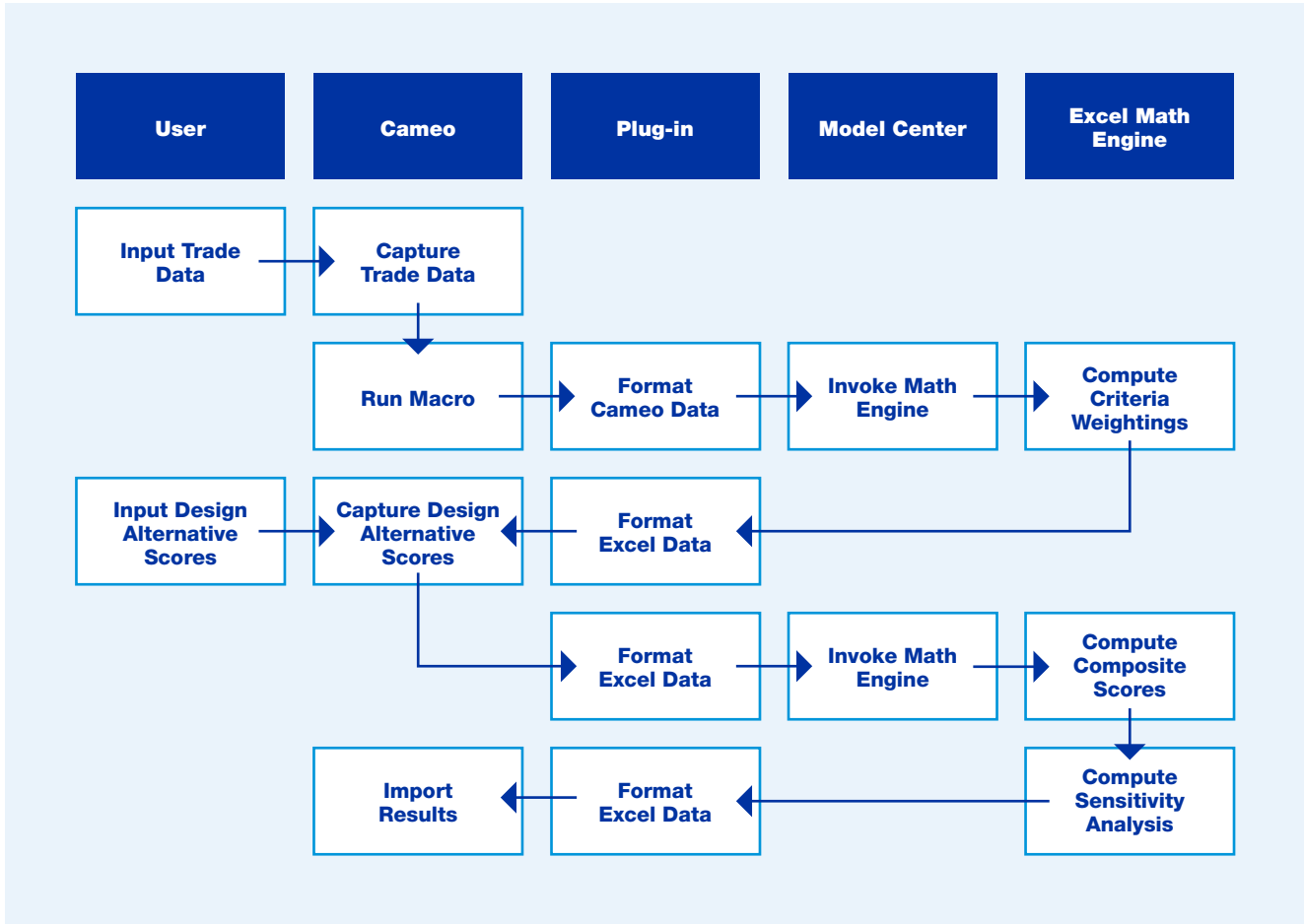
FIGURE 1. MBTIF structure
