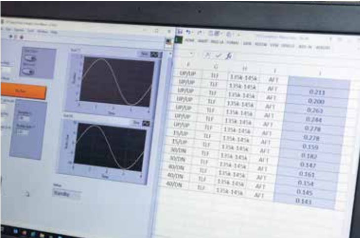
DRI CLOSE-UP The DRI rudder signal can be manipulated using a custom DRI software client, which controls the Fault and Function Generator system commonly used for other flight testing.
